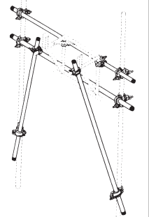
SCAFFOLD OUTRIGGER
