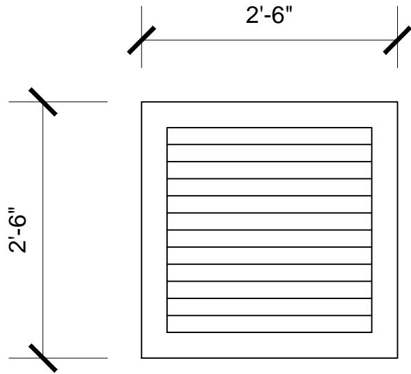
TYPICAL WALL MOUNTED LOUVER PLAN VIEW
