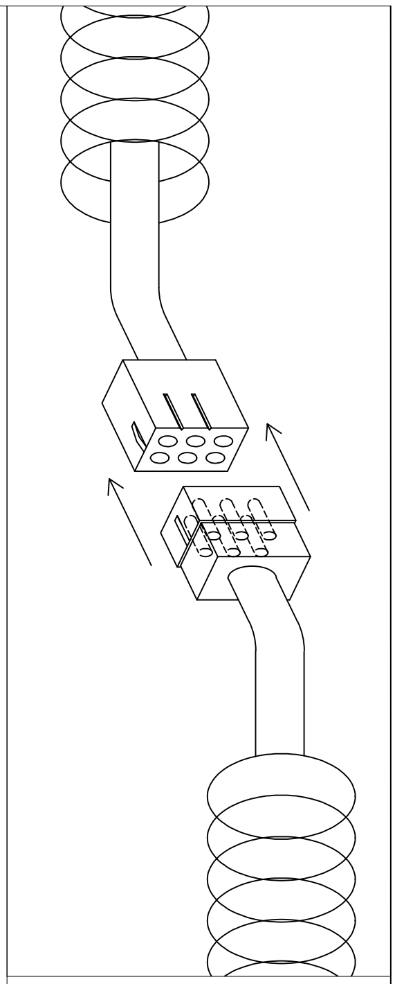
"DETAIL A" QUICK CONNECT FROM DOOR TO DOOR
