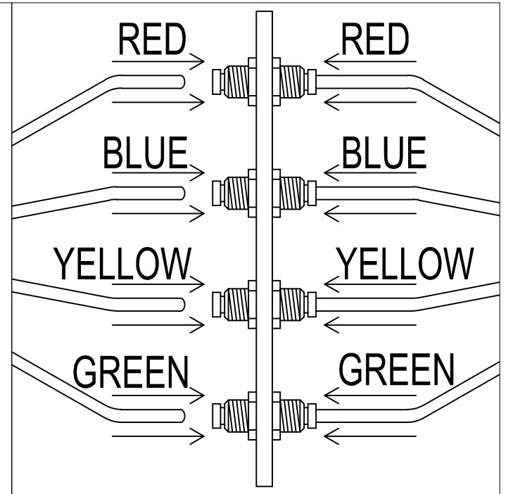
DETAIL "A" (PUSH TO CONNECT)
