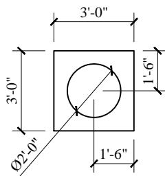
FLOOR RETAINING FLANGE
