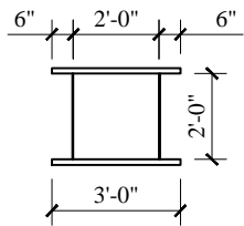
TYPICAL FLOOR FRAME
