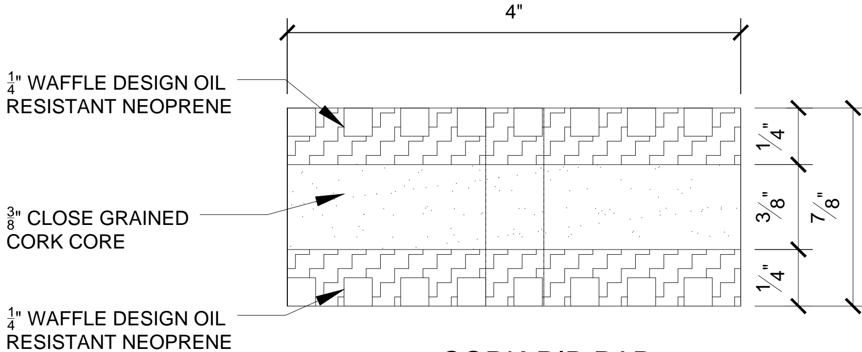
CORK-RIB PAD SIDE VIEW
