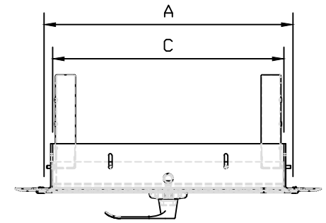
*TOP VIEW FOR 24" X 24" DOOR
